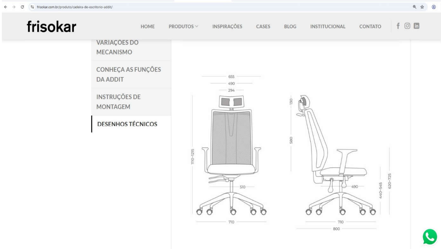
Figura 3 - Dimensional (site)
